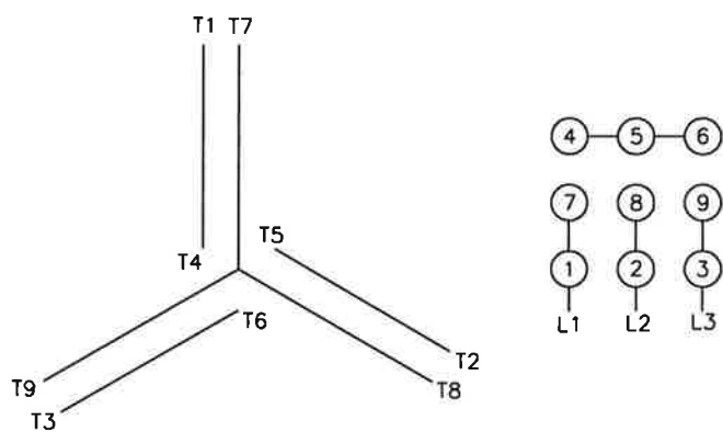
Low Voltage Wye
